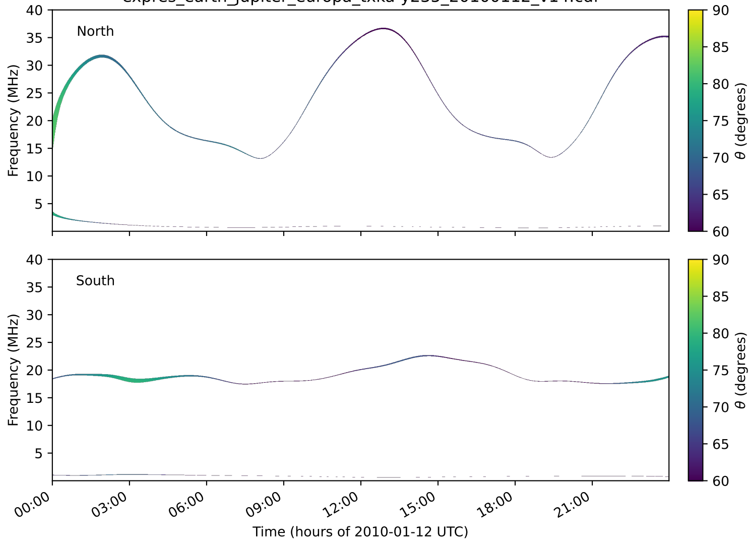
expres_earth_jupiter_europa_txka-y235_20100112_v14.cdf
