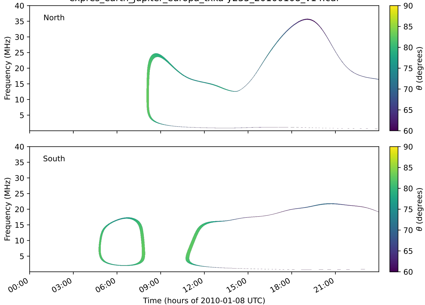
expres_earth_jupiter_europa_txka-y235_20100108_v14.cdf
