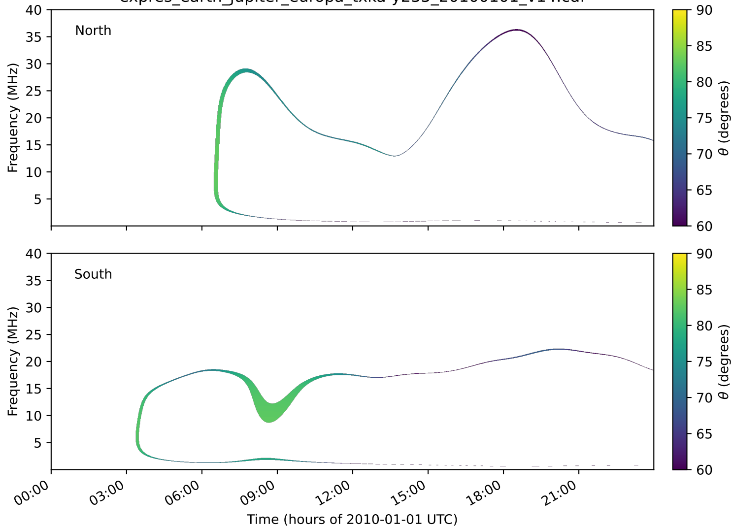
expres_earth_jupiter_europa_txka-y235_20100101_v14.cdf
