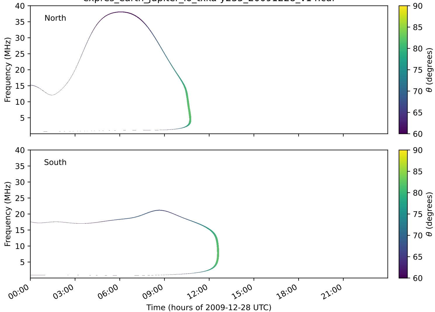
expres_earth_jupiter_io_txka-y235_20091228_v14.cdf
