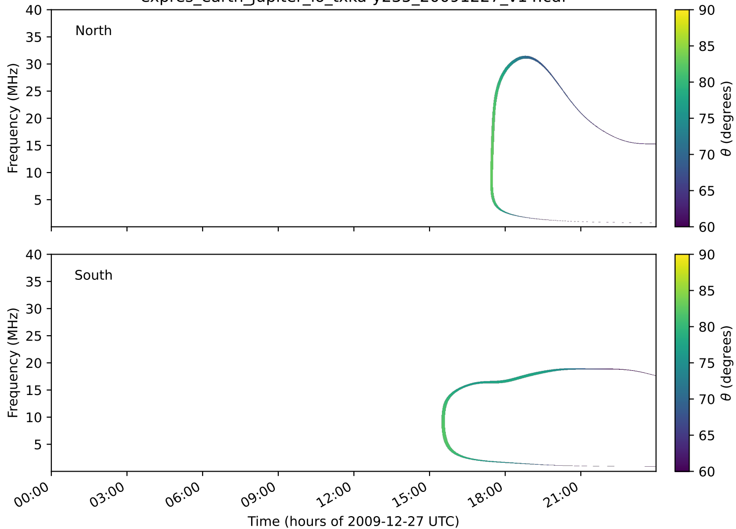
expres_earth_jupiter_io_txka-y235_20091227_v14.cdf
