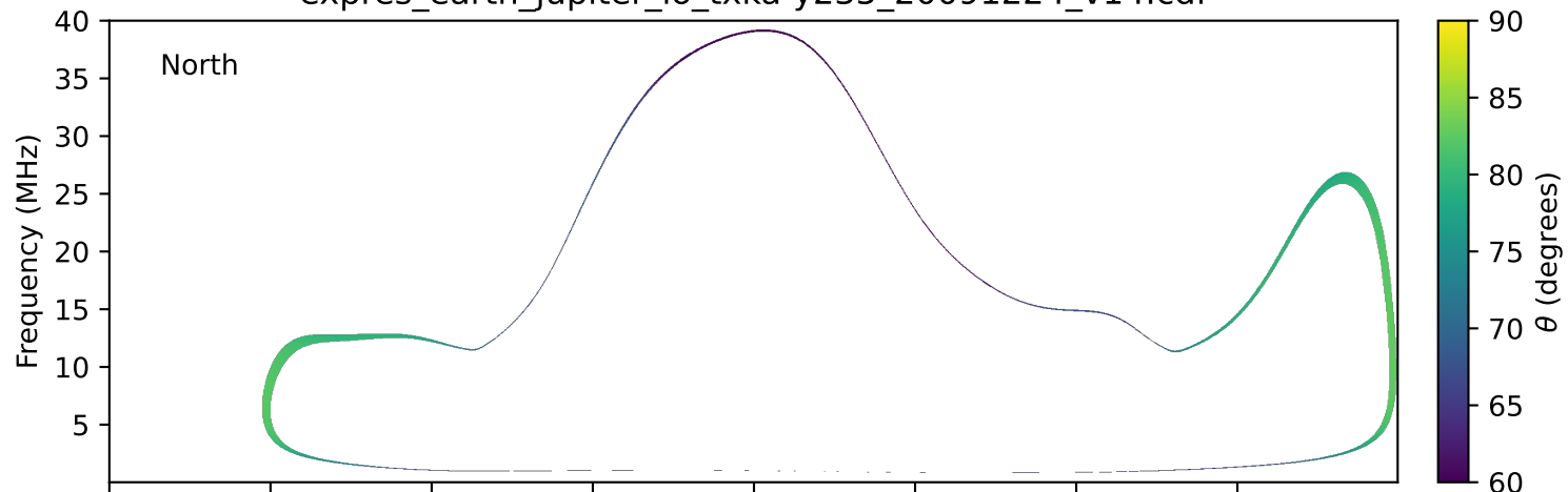
expres_earth_jupiter_io_txka-y235_20091224_v14.cdf
