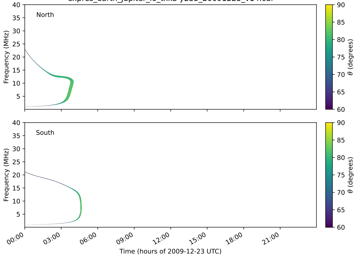
expres_earth_jupiter_io_txka-y235_20091223_v14.cdf
