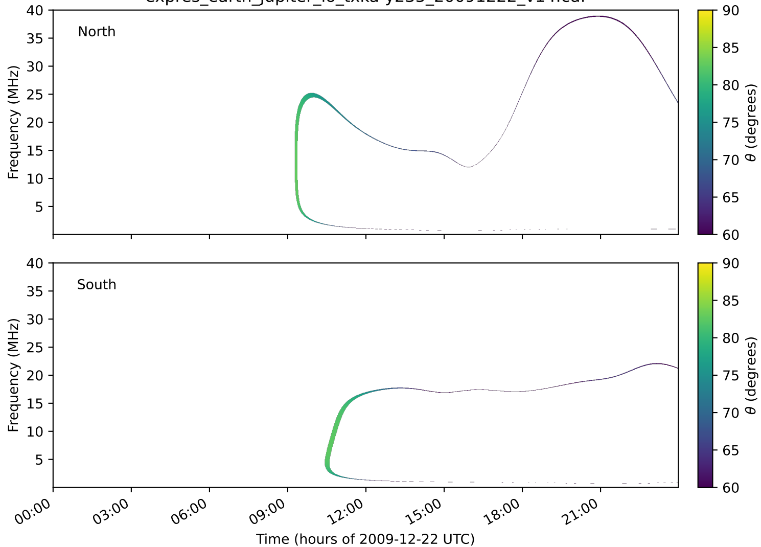
expres_earth_jupiter_io_txka-y235_20091222_v14.cdf
