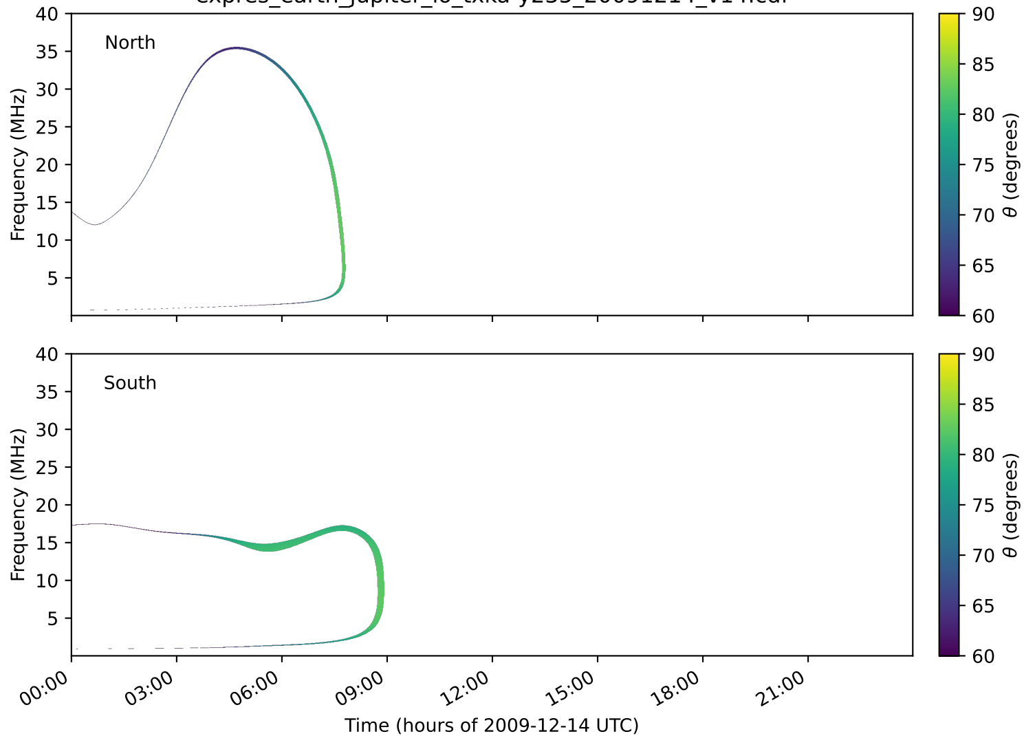
expres_earth_jupiter_io_txka-y235_20091214_v14.cdf
