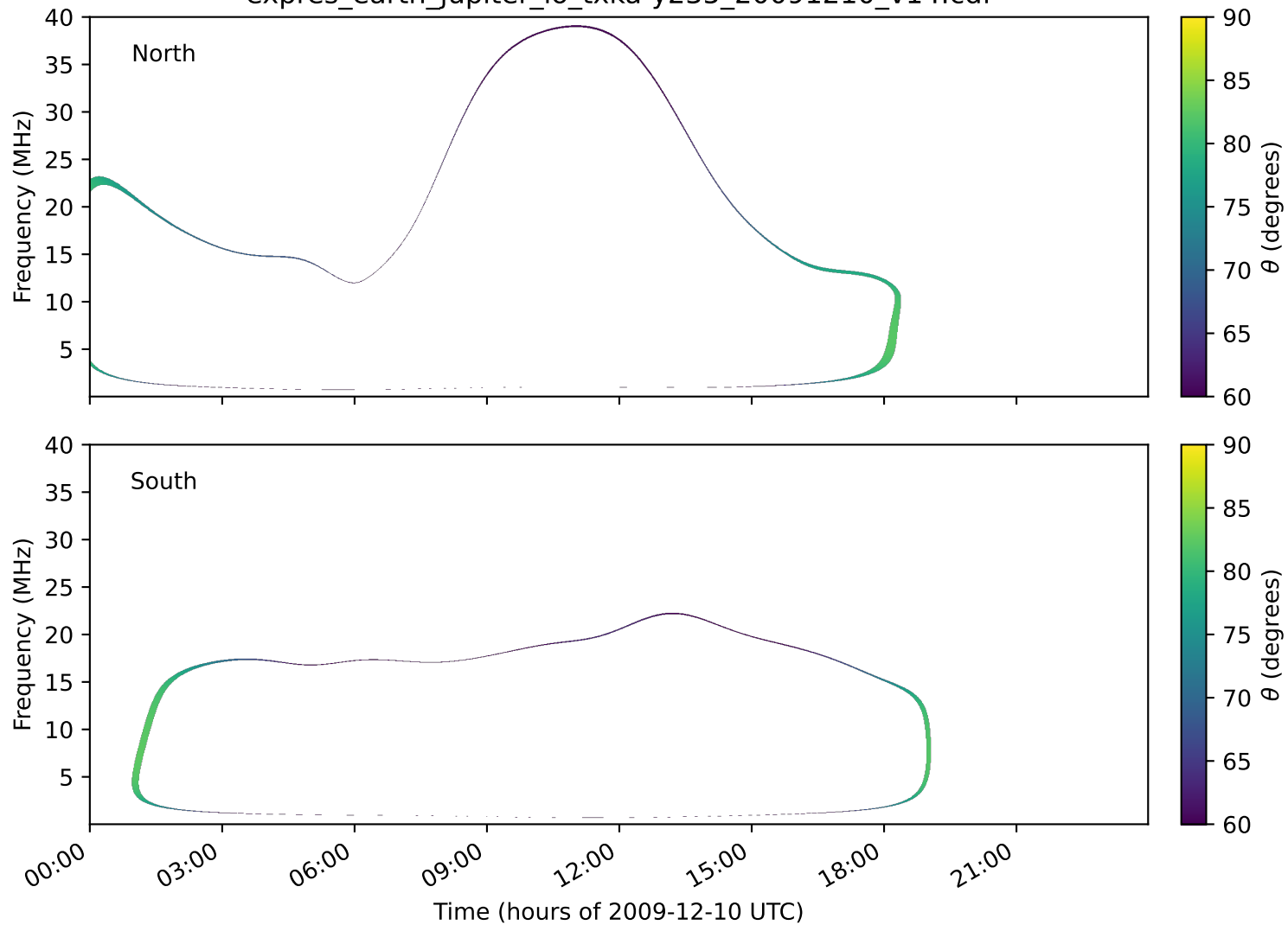
expres_earth_jupiter_io_txka-y235_20091210_v14.cdf
