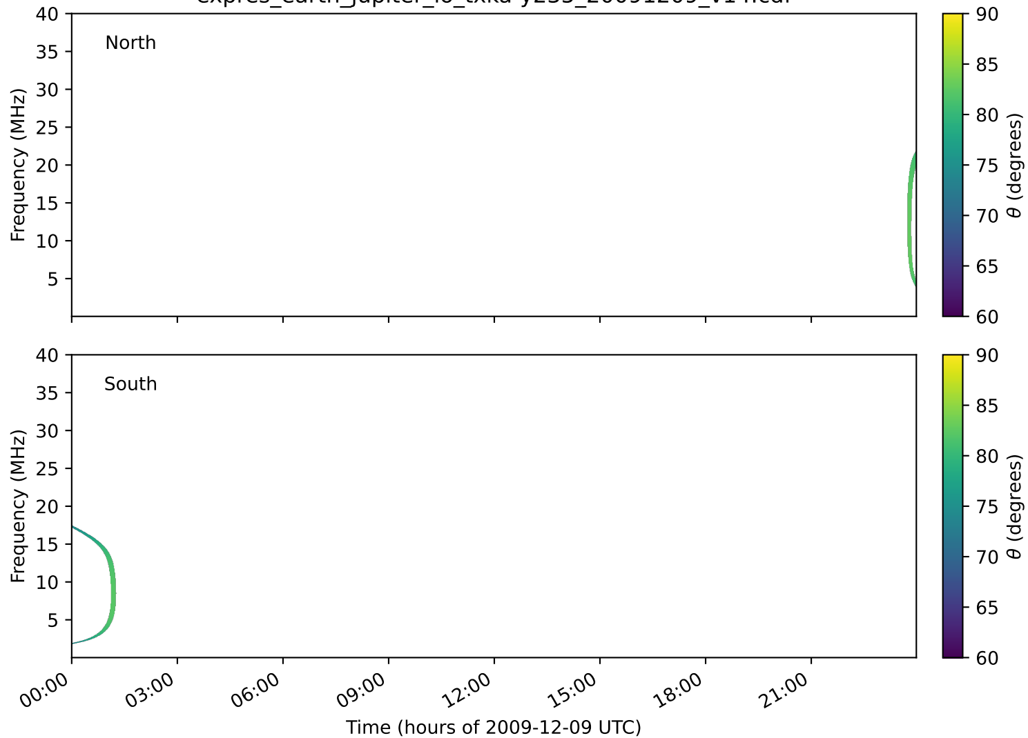
expres_earth_jupiter_io_txka-y235_20091209_v14.cdf
