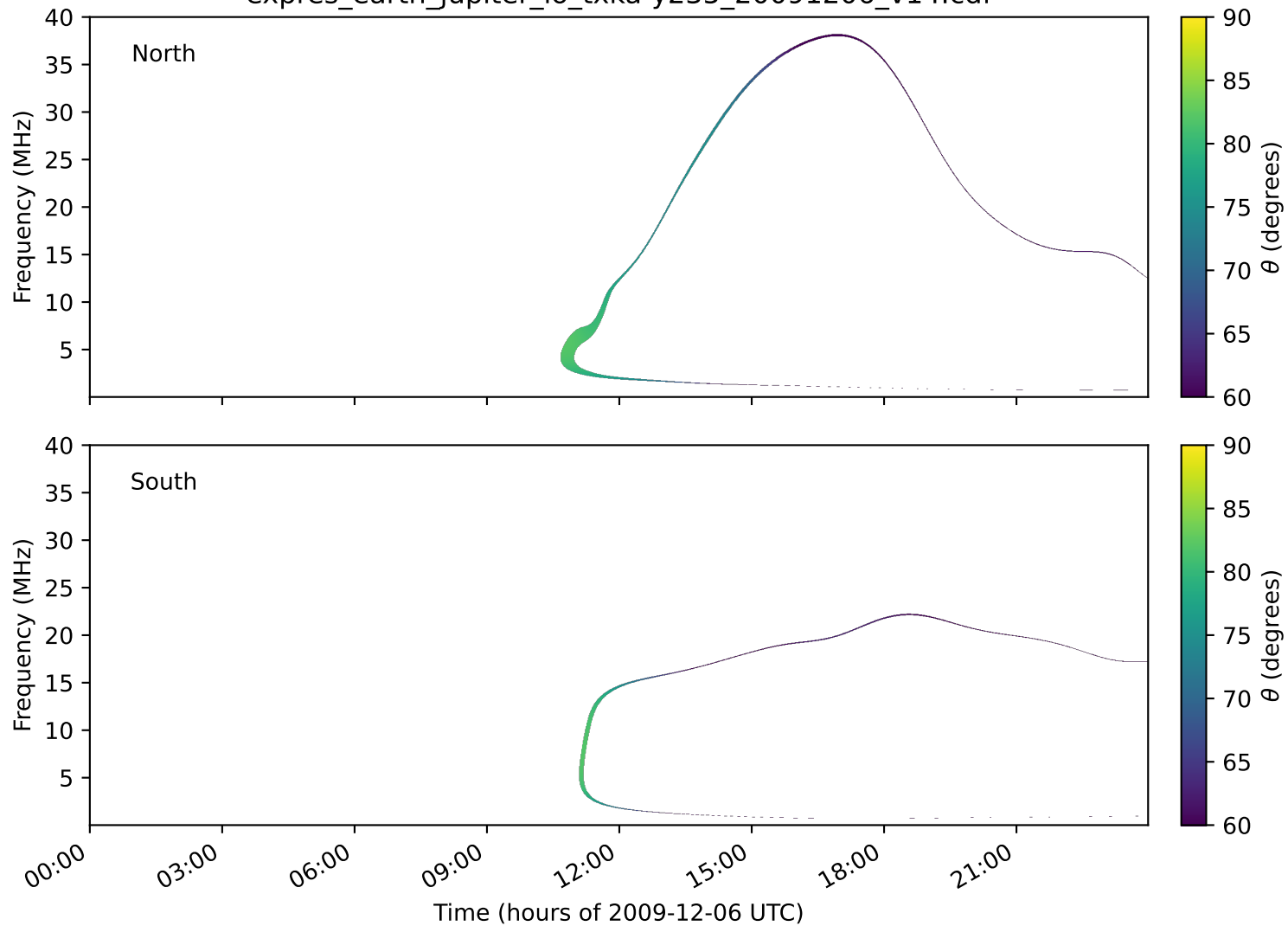
expres_earth_jupiter_io_txka-y235_20091206_v14.cdf
