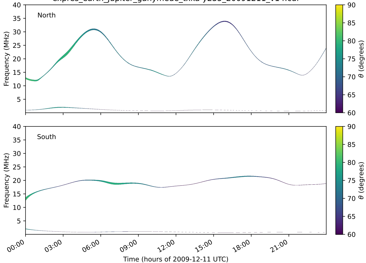
expres_earth_jupiter_ganymede_txka-y235_20091211_v14.cdf
