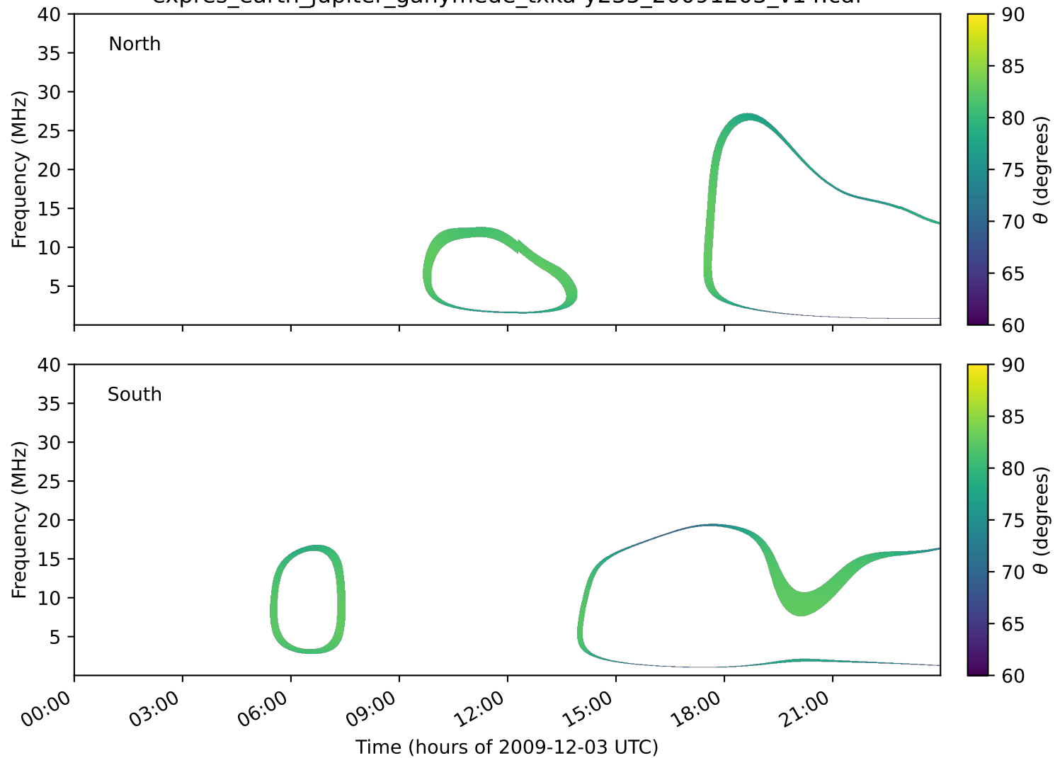
expres_earth_jupiter_ganymede_txka-y235_20091203_v14.cdf
