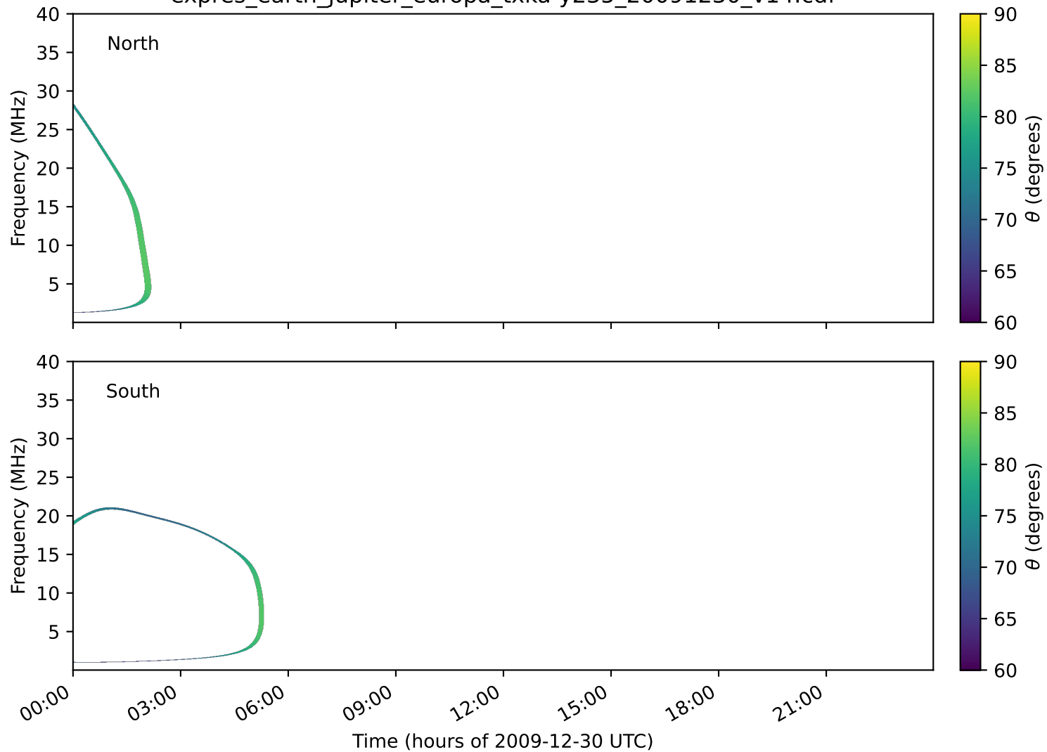
expres_earth_jupiter_europa_txka-y235_20091230_v14.cdf
