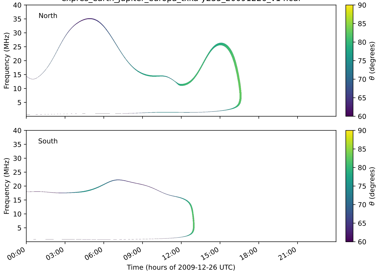
expres_earth_jupiter_europa_txka-y235_20091226_v14.cdf
