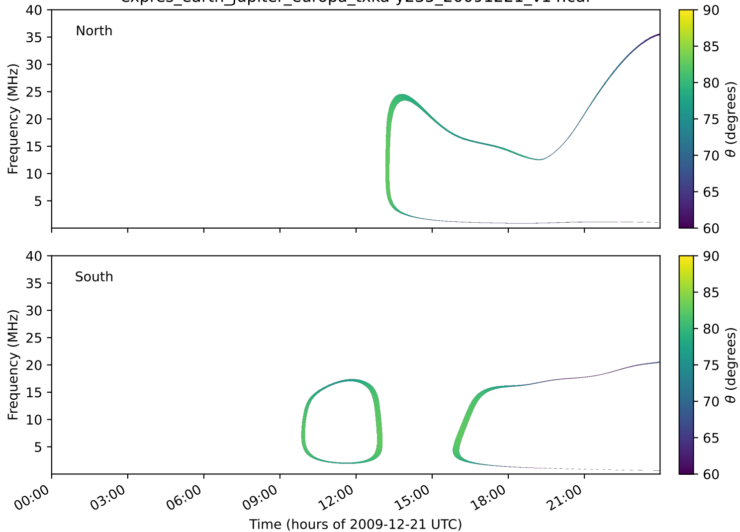
expres_earth_jupiter_europa_txka-y235_20091221_v14.cdf
