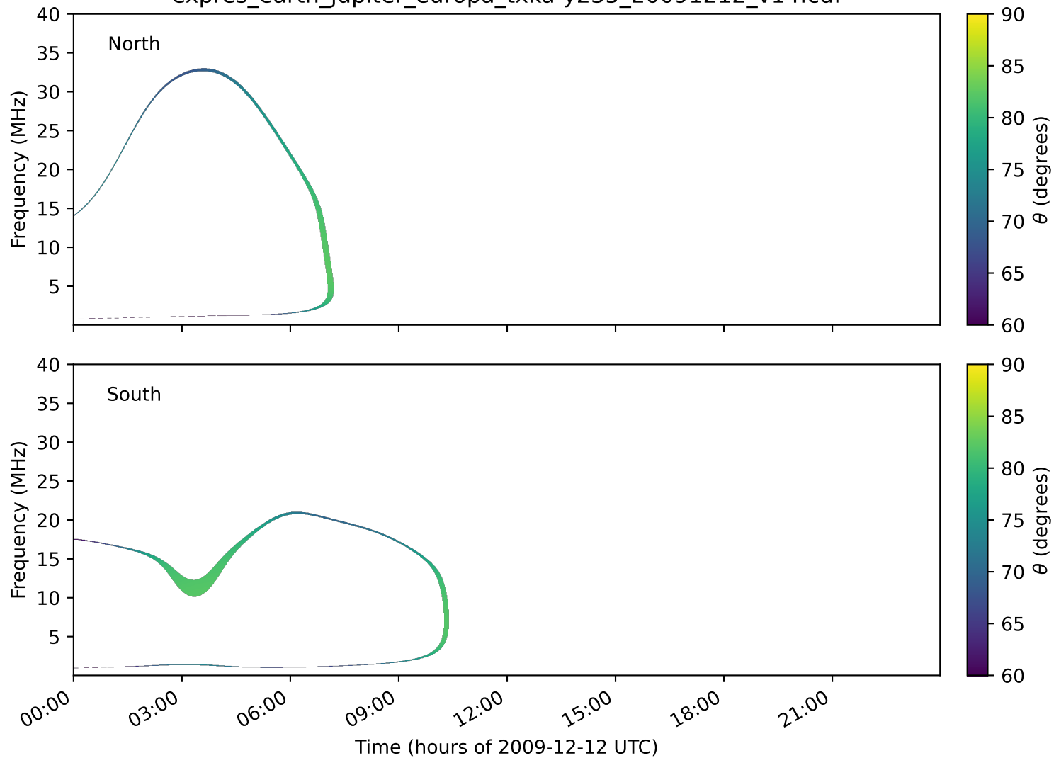
expres_earth_jupiter_europa_txka-y235_20091212_v14.cdf
