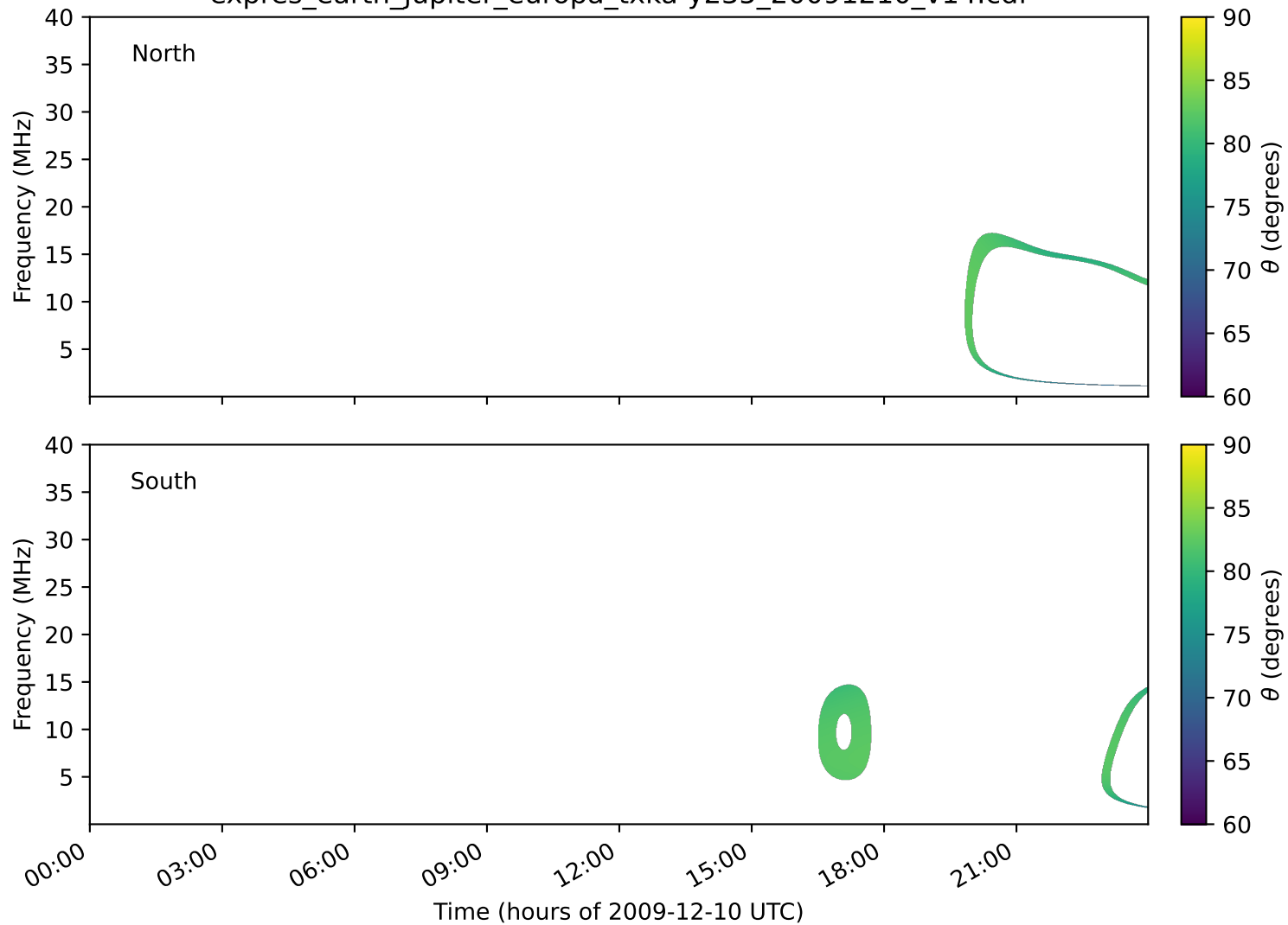
expres_earth_jupiter_europa_txka-y235_20091210_v14.cdf
