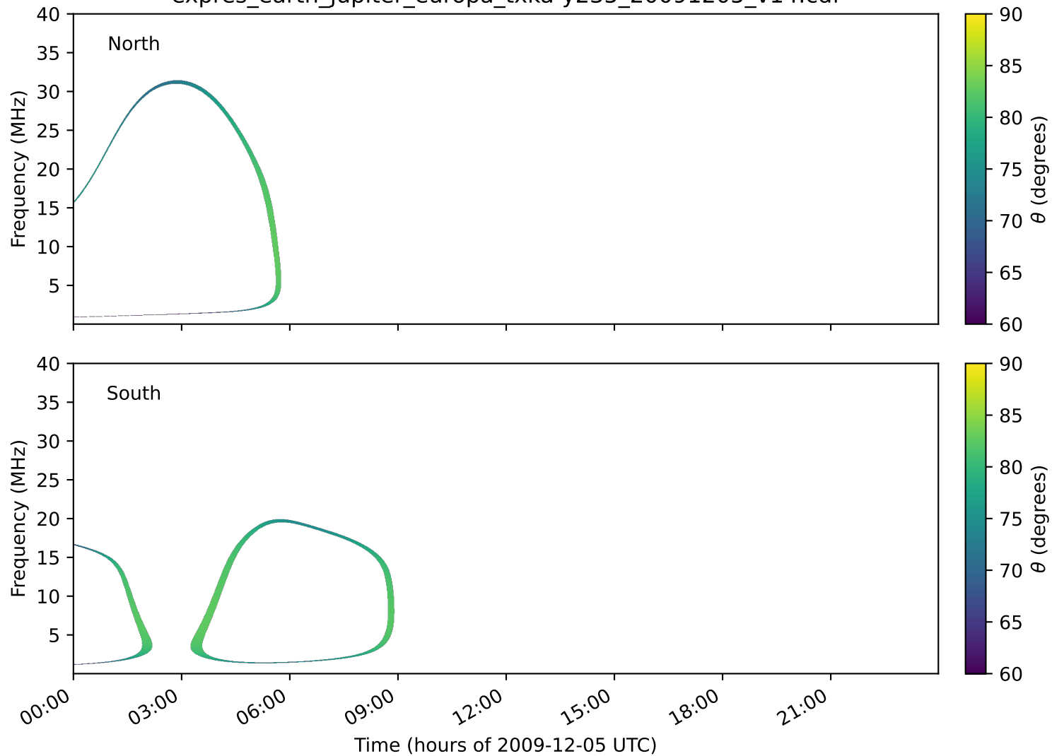
expres_earth_jupiter_europa_txka-y235_20091205_v14.cdf
