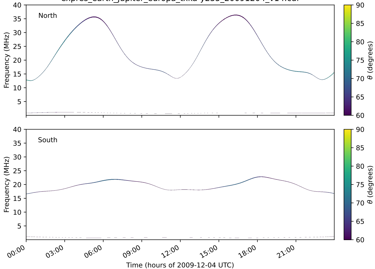
expres_earth_jupiter_europa_txka-y235_20091204_v14.cdf
