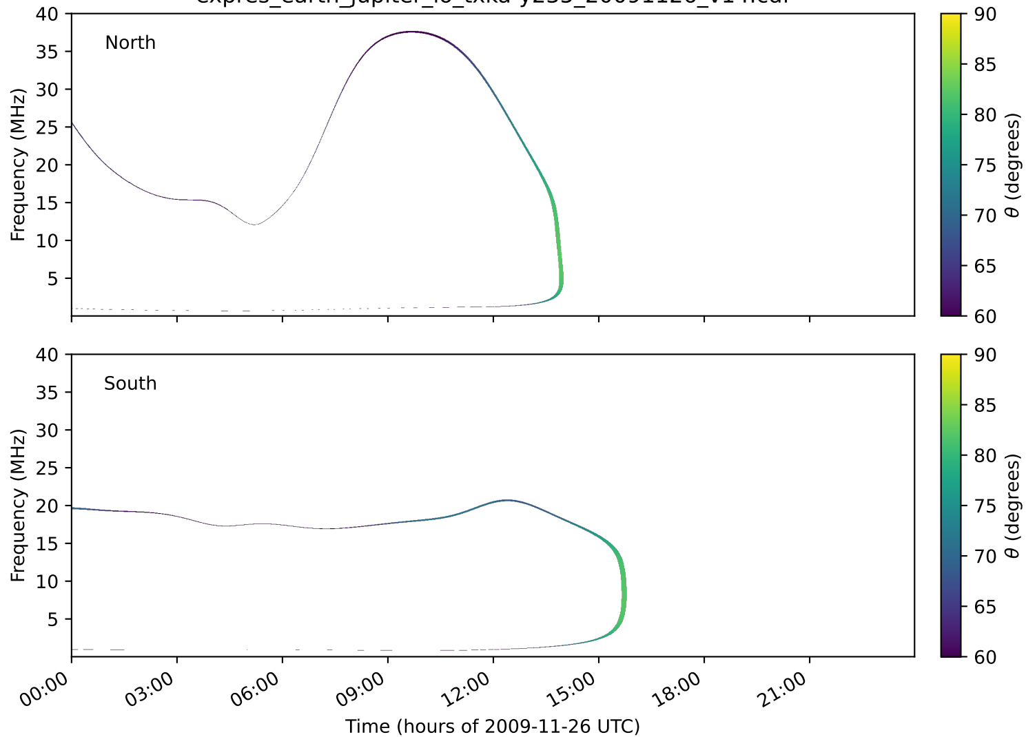
expres_earth_jupiter_io_txka-y235_20091126_v14.cdf
