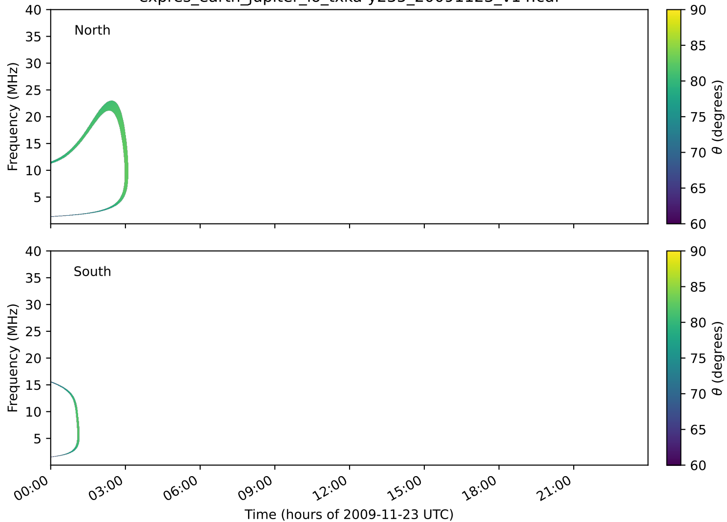
expres_earth_jupiter_io_txka-y235_20091123_v14.cdf
