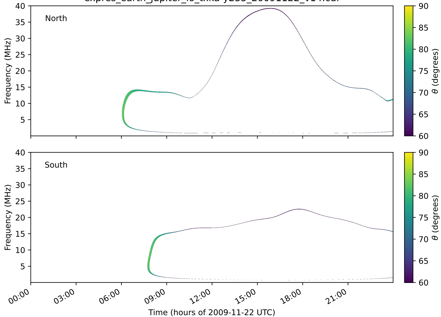
expres_earth_jupiter_io_txka-y235_20091122_v14.cdf
