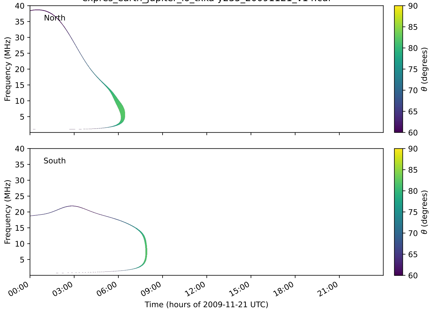
expres_earth_jupiter_io_txka-y235_20091121_v14.cdf
