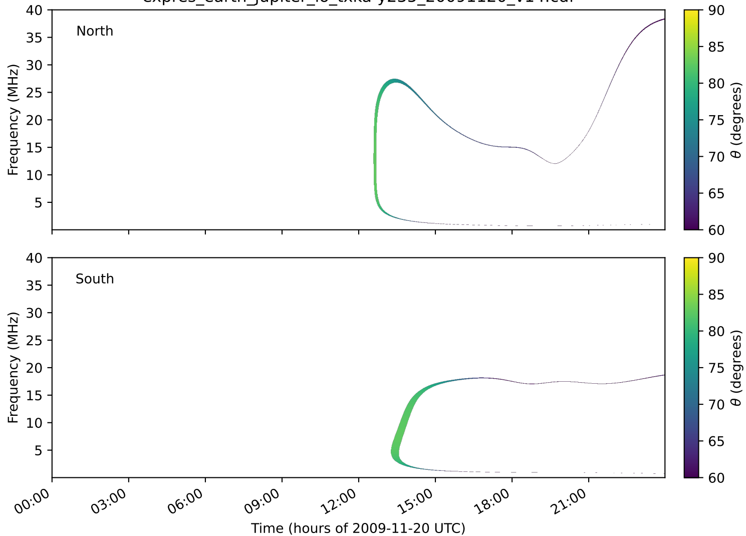
expres_earth_jupiter_io_txka-y235_20091120_v14.cdf
