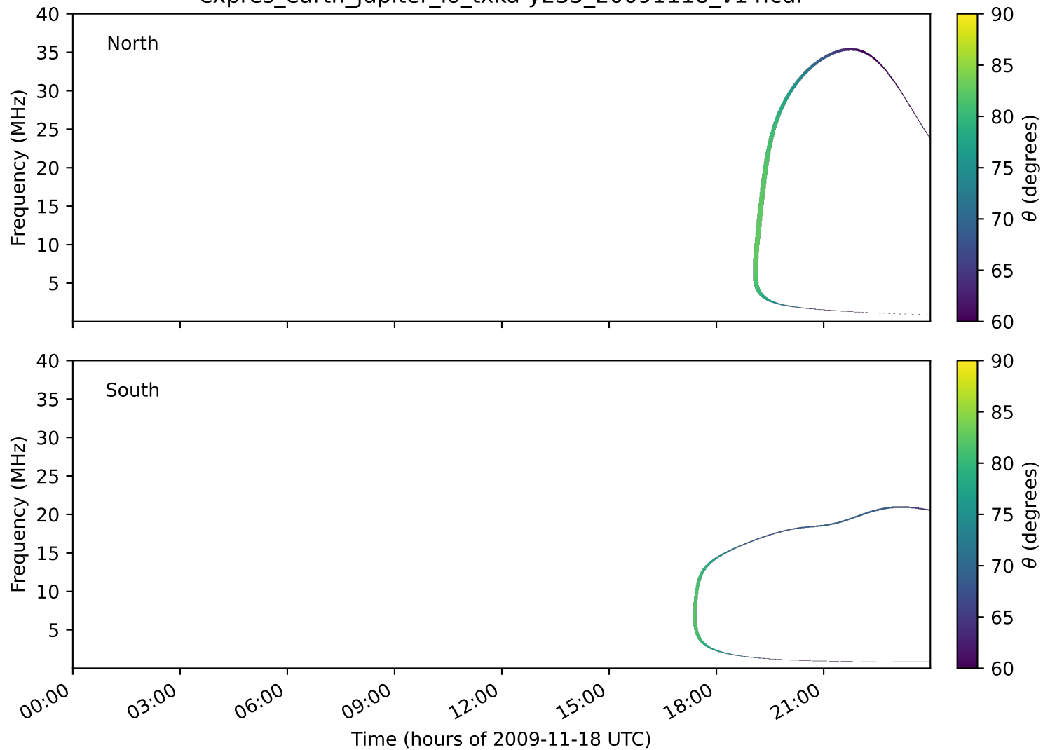
expres_earth_jupiter_io_txka-y235_20091118_v14.cdf
