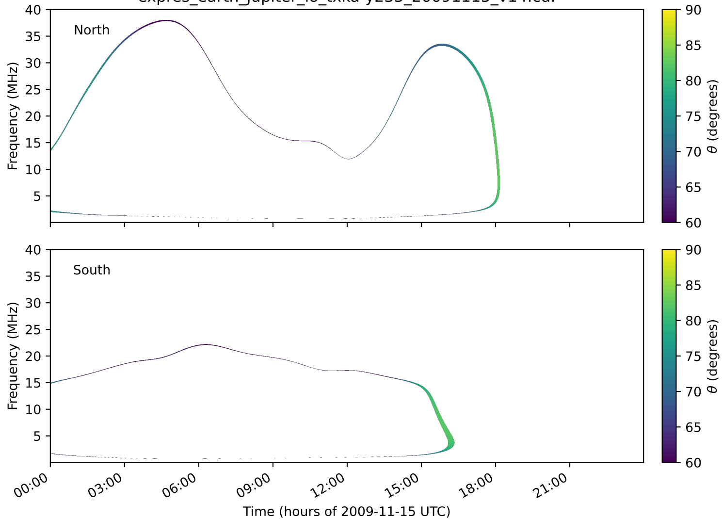
expres_earth_jupiter_io_txka-y235_20091115_v14.cdf
