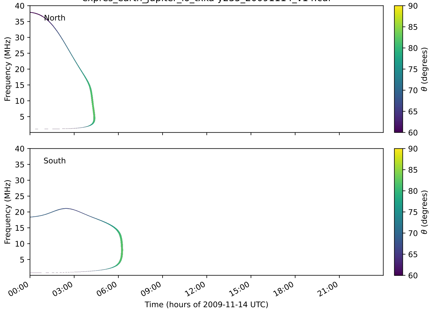
expres_earth_jupiter_io_txka-y235_20091114_v14.cdf
