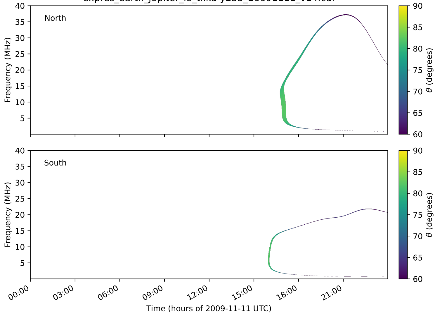
expres_earth_jupiter_io_txka-y235_20091111_v14.cdf
