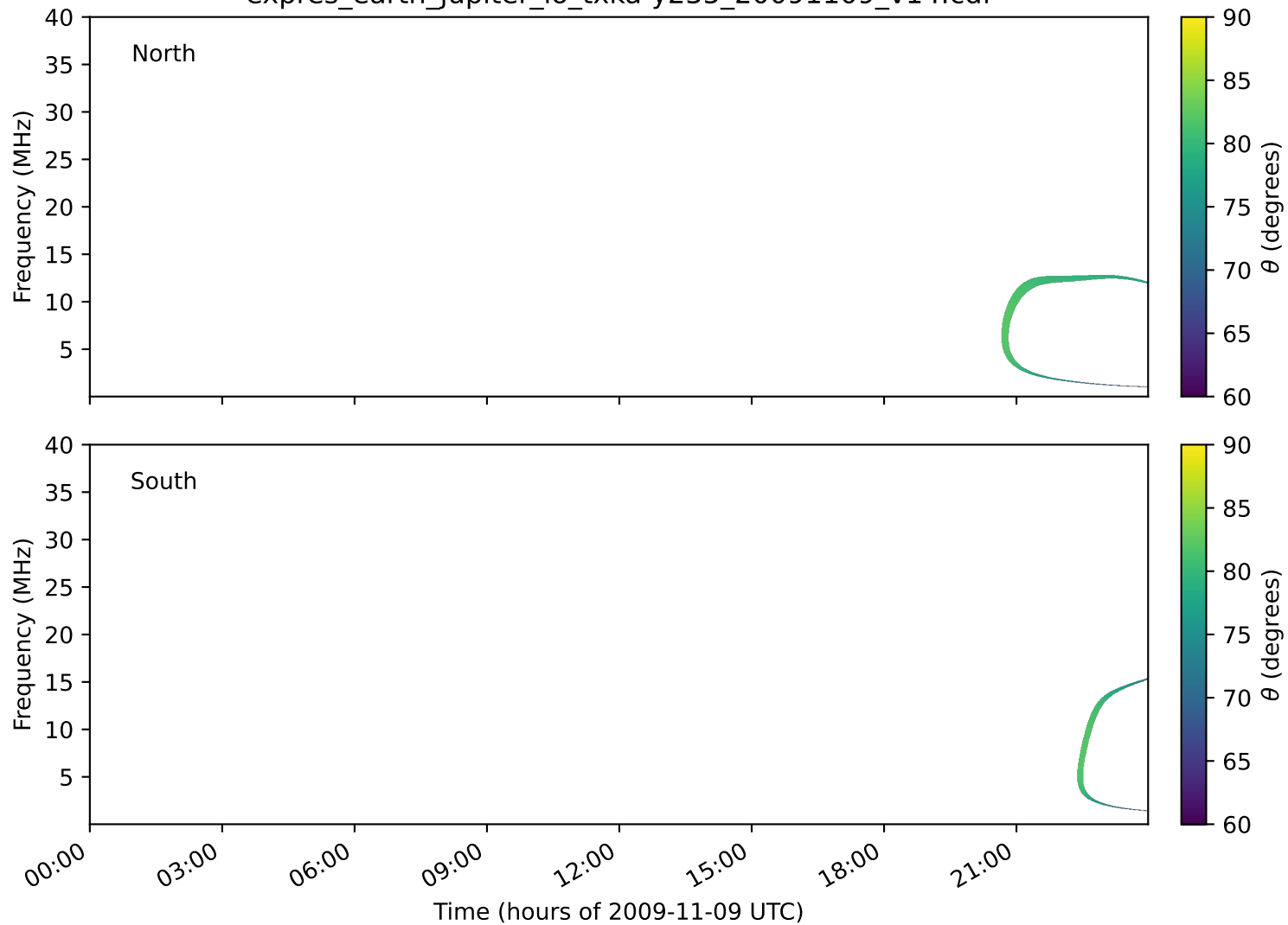
expres_earth_jupiter_io_txka-y235_20091109_v14.cdf
