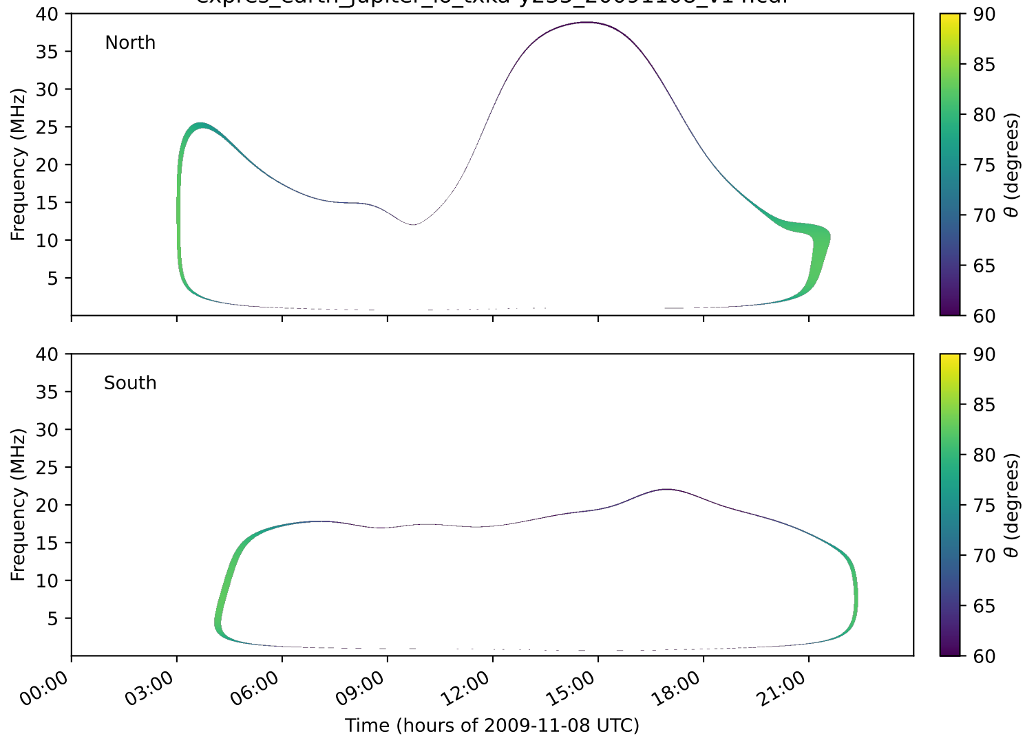
expres_earth_jupiter_io_txka-y235_20091108_v14.cdf
