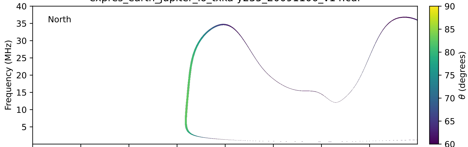
expres_earth_jupiter_io_txka-y235_20091106_v14.cdf
