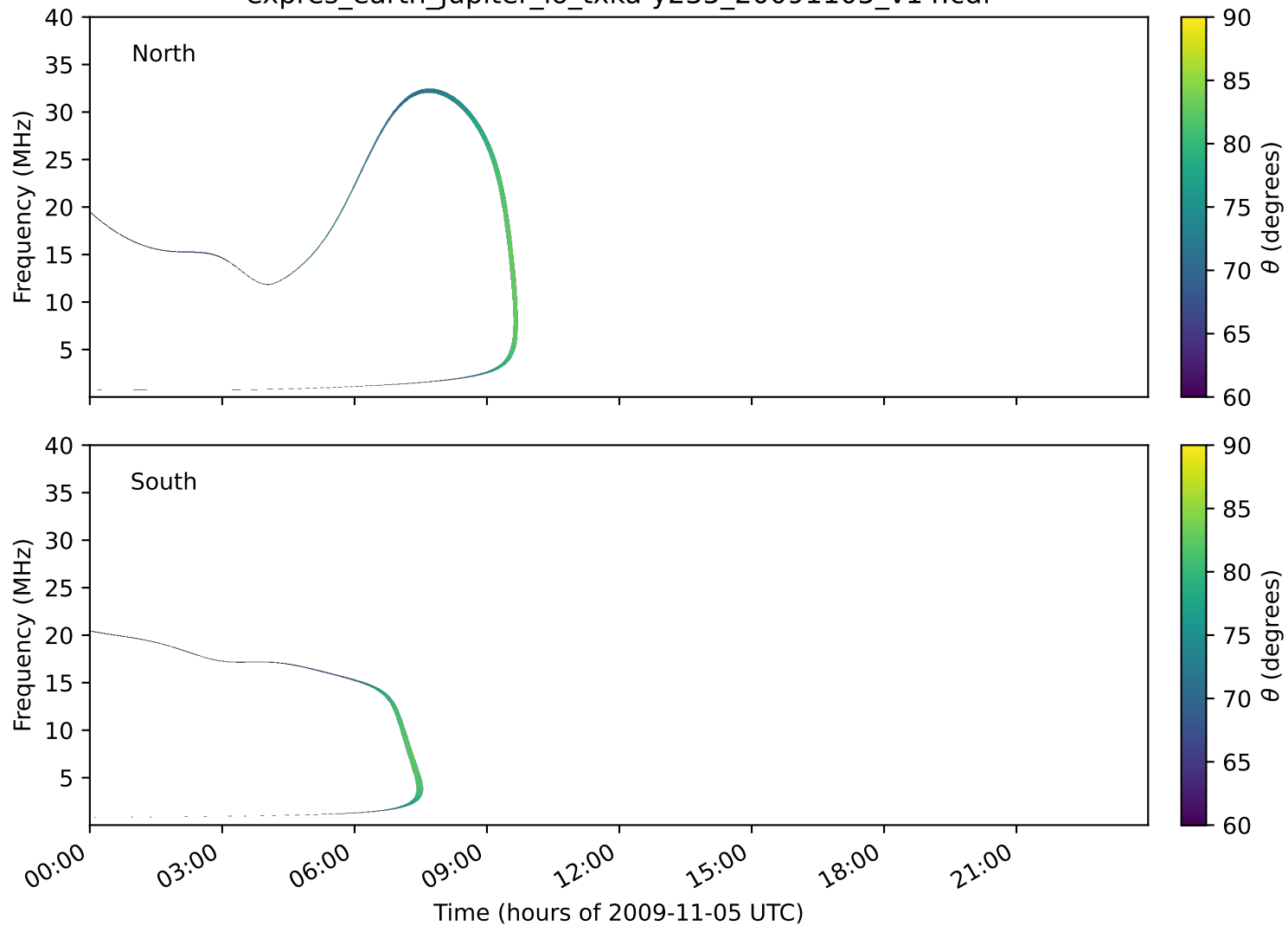
expres_earth_jupiter_io_txka-y235_20091105_v14.cdf
