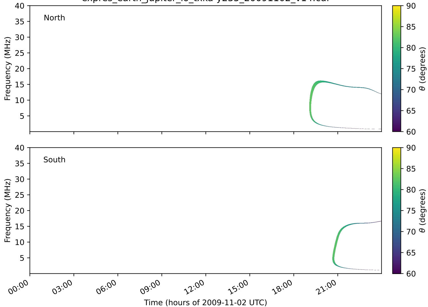
expres_earth_jupiter_io_txka-y235_20091102_v14.cdf
