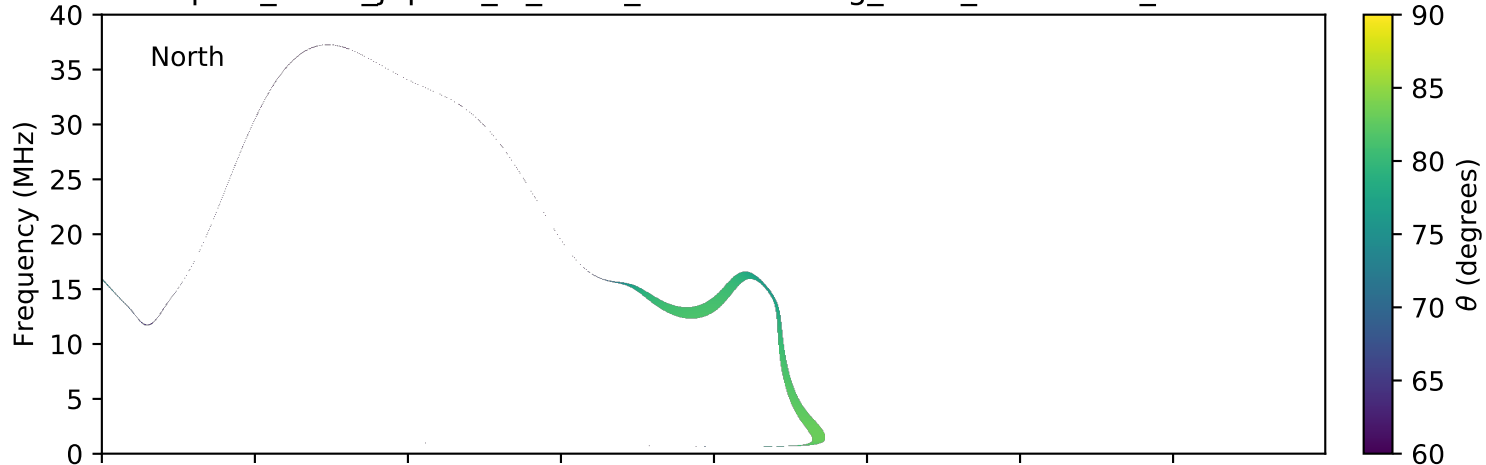
expres_earth_jupiter_io_isaac_lossc-wid1deg_3kev_20091103_v01.cdf
