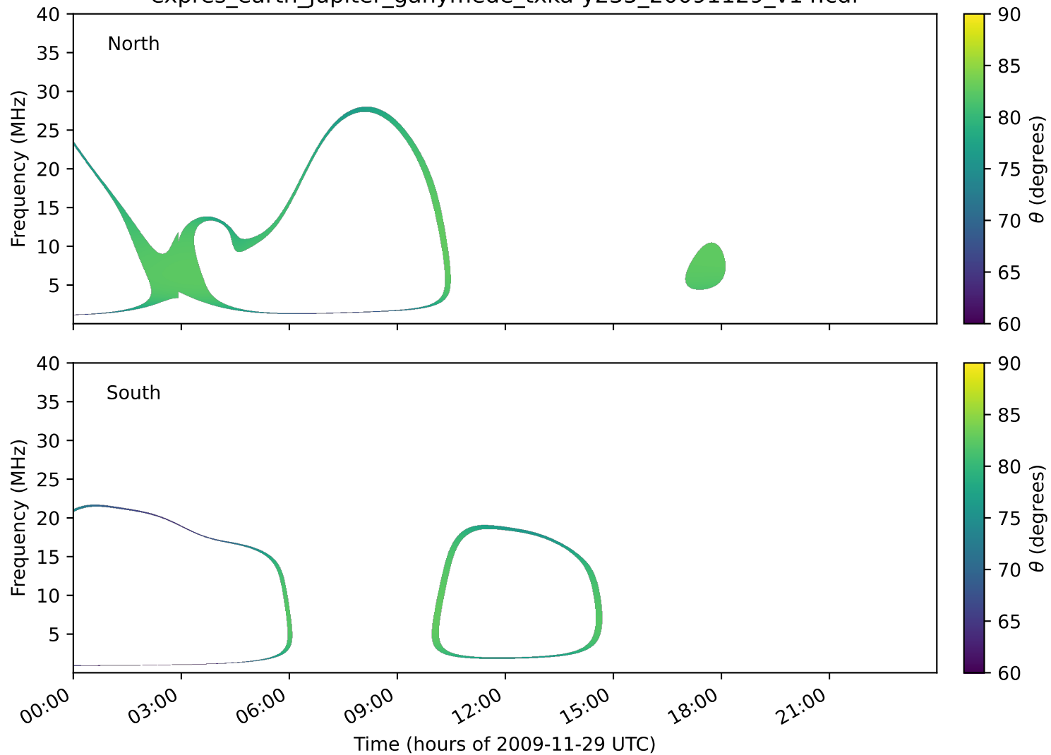
expres_earth_jupiter_ganymede_txka-y235_20091129_v14.cdf
