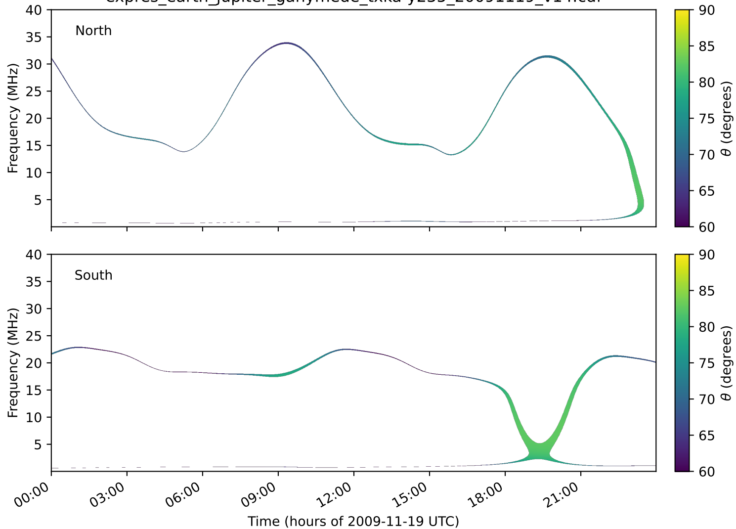
expres_earth_jupiter_ganymede_txka-y235_20091119_v14.cdf
