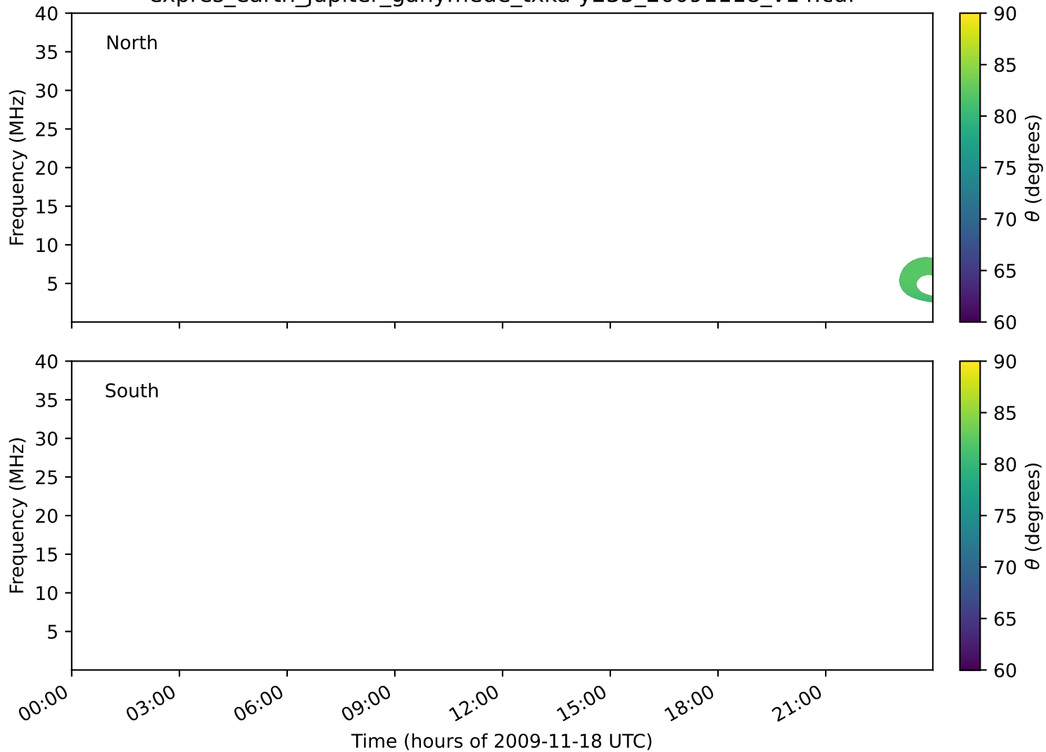
expres_earth_jupiter_ganymede_txka-y235_20091118_v14.cdf
