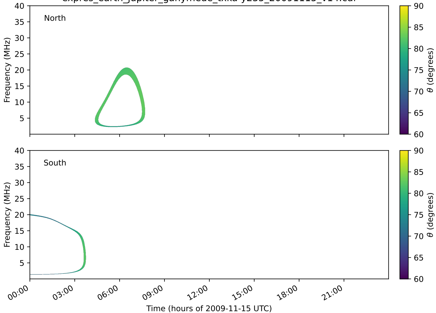
expres_earth_jupiter_ganymede_txka-y235_20091115_v14.cdf
