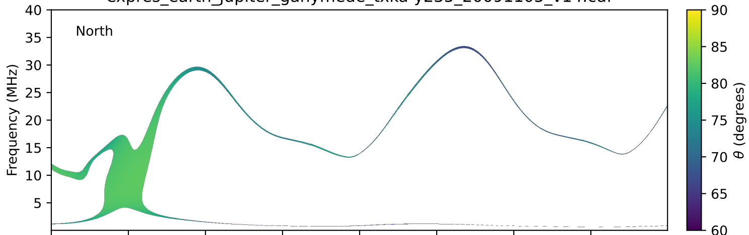
expres_earth_jupiter_ganymede_txka-y235_20091105_v14.cdf
