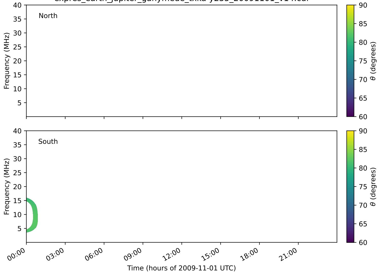
expres_earth_jupiter_ganymede_txka-y235_20091101_v14.cdf
