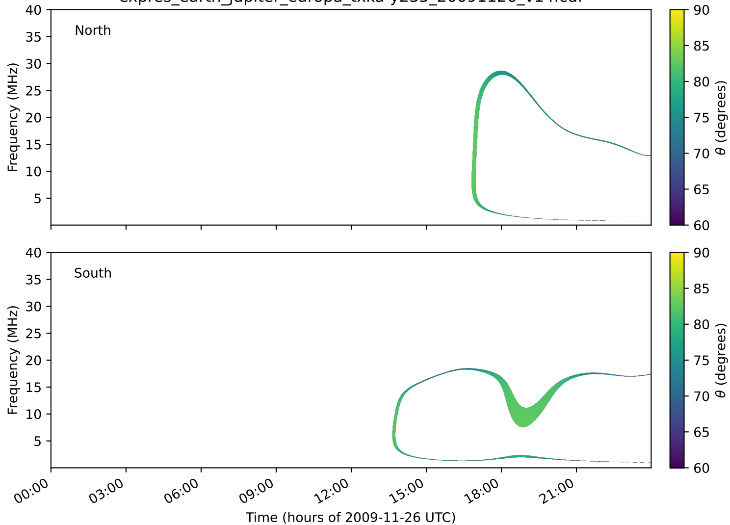
expres_earth_jupiter_europa_txka-y235_20091126_v14.cdf
