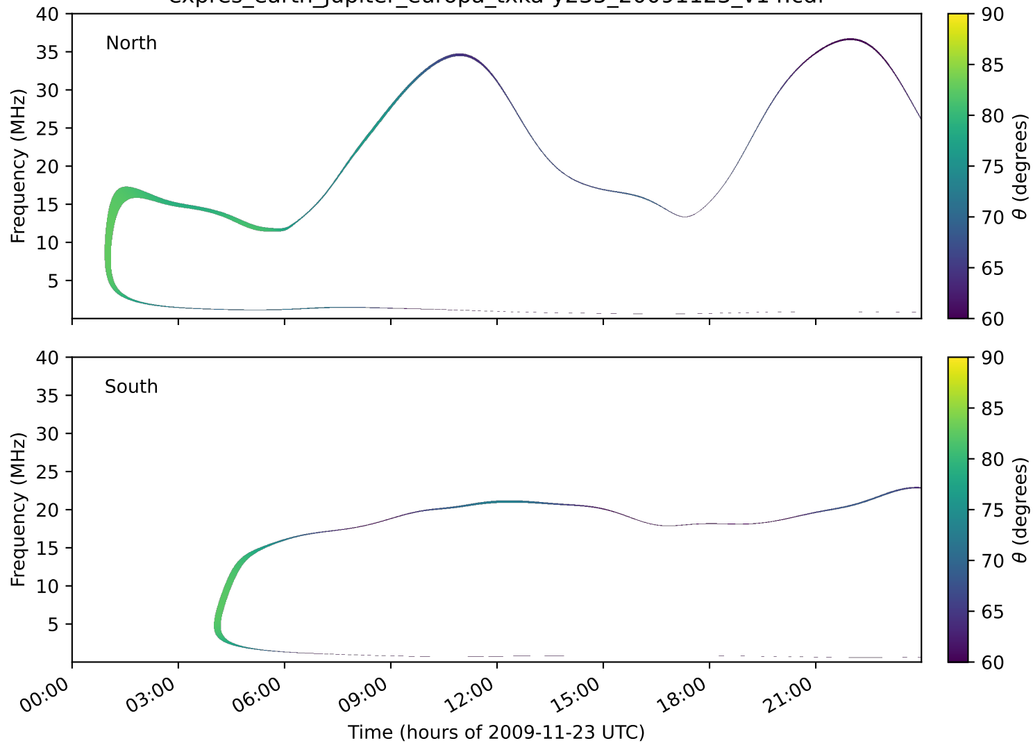
expres_earth_jupiter_europa_txka-y235_20091123_v14.cdf
