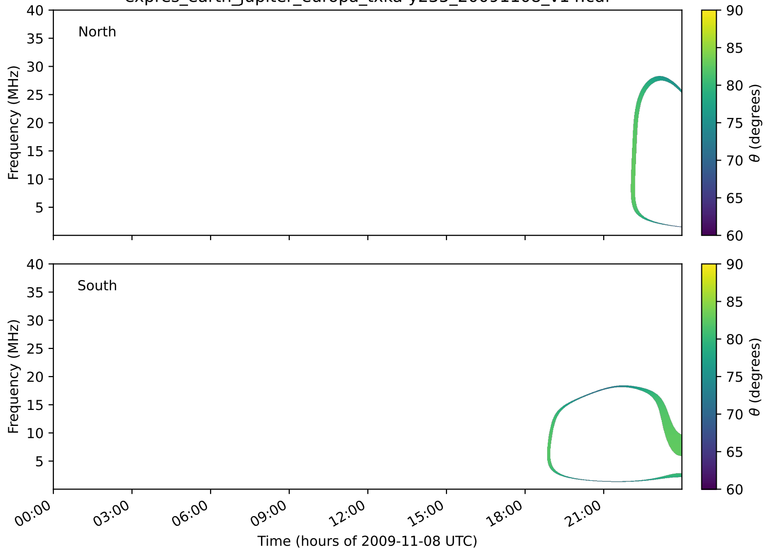
expres_earth_jupiter_europa_txka-y235_20091108_v14.cdf
