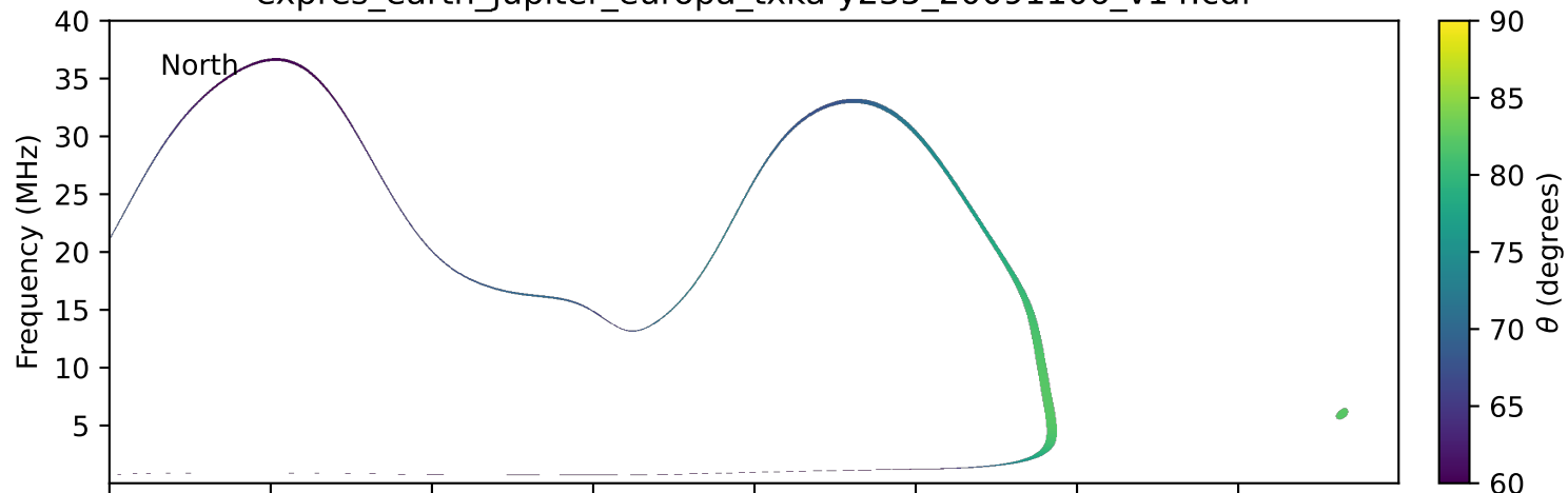
expres_earth_jupiter_europa_txka-y235_20091106_v14.cdf
