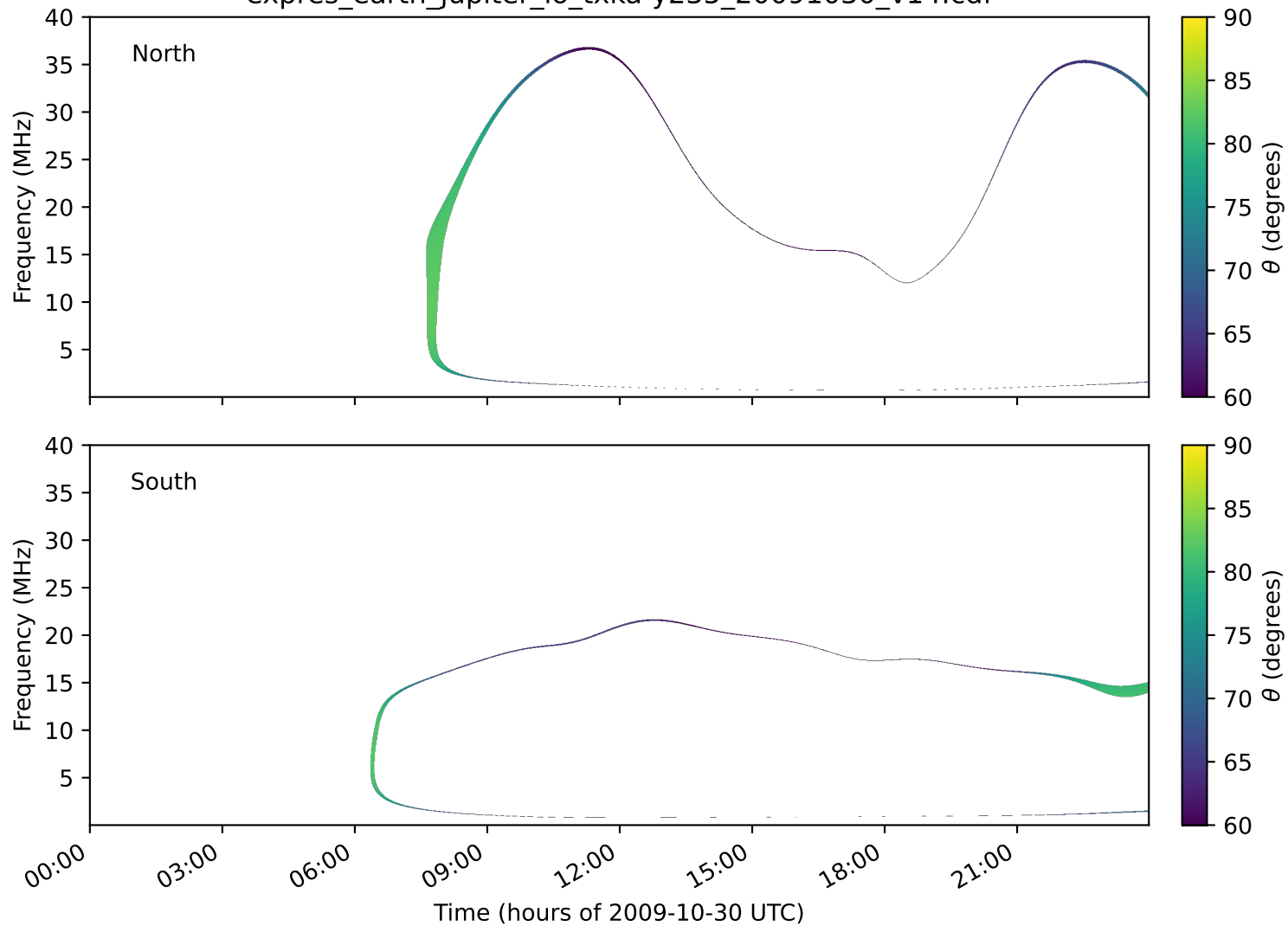
expres_earth_jupiter_io_txka-y235_20091030_v14.cdf
