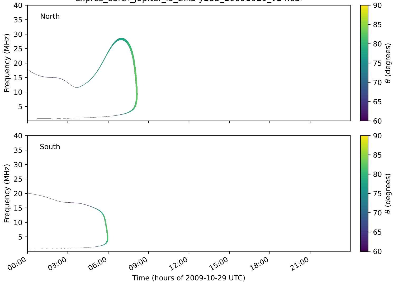
expres_earth_jupiter_io_txka-y235_20091029_v14.cdf
