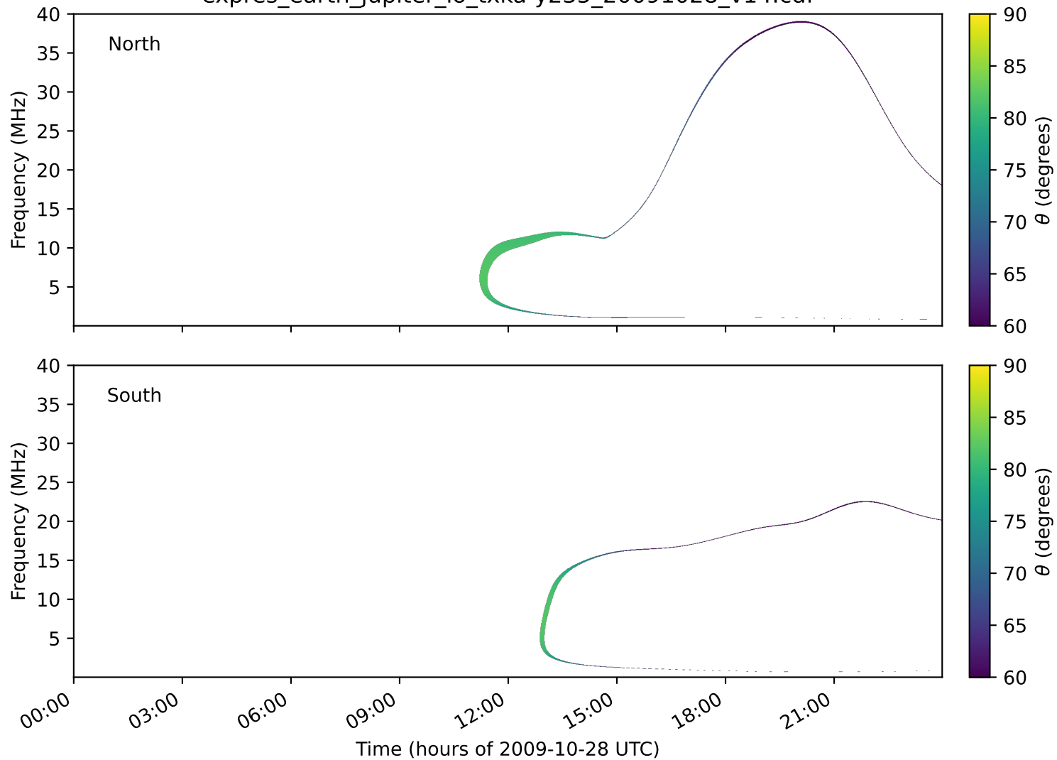
expres_earth_jupiter_io_txka-y235_20091028_v14.cdf
