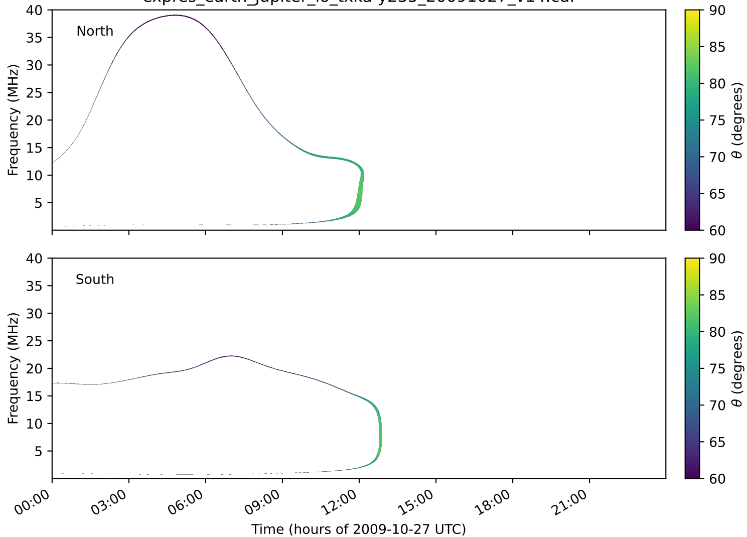
expres_earth_jupiter_io_txka-y235_20091027_v14.cdf
